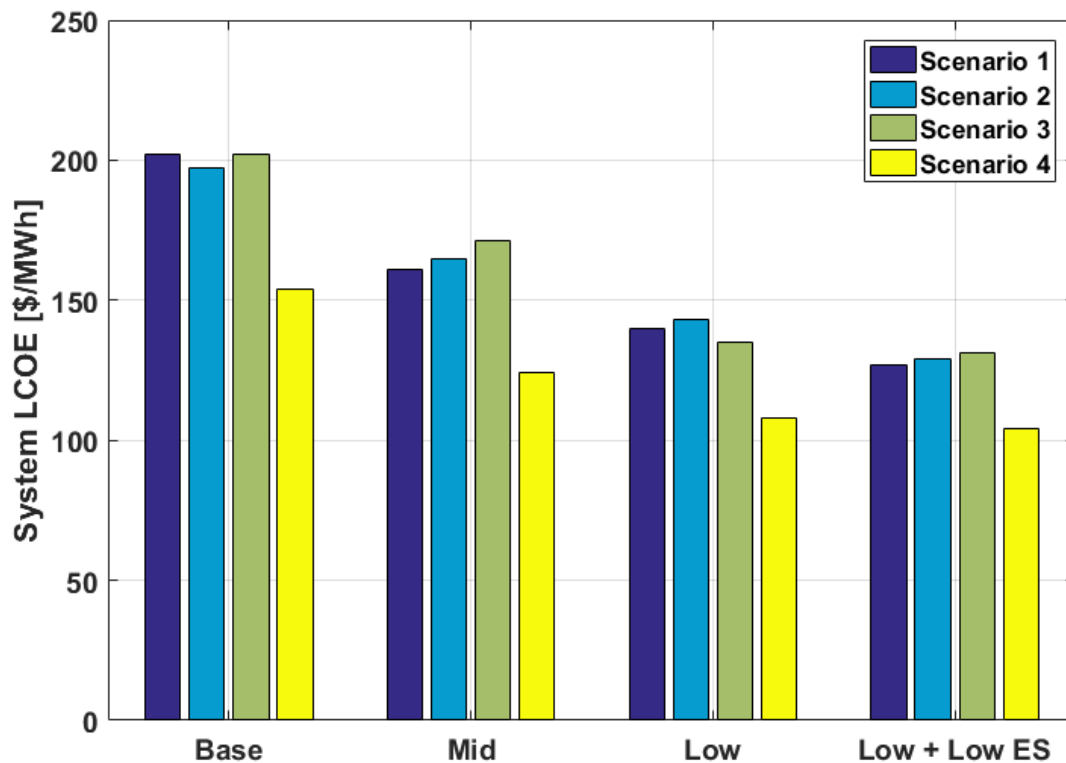
Figure 5 – Sensitivity of the lowest LCOE values in each scenario to projected future costs of energy resources using a 99.5% zero-carbon threshold. “Base” = Cost data inputs from the NREL ATB dataset for the base year of 2017. “Mid” = Cost data inputs from the NREL ATB Mid-case for the year 2045. “Low” = Cost data inputs from the NREL ATB Low-case for the year 2045. “Low + Low ES” = Same as the “Low” case, but additionally includes the projected cost reductions in energy storage system capital costs.
