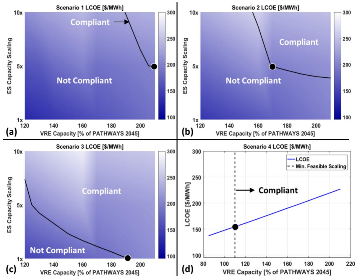
Figure 2 - Levelized Cost of Electricity (LCOE) values for different realizations of each narrative scenario using a 99.5% zero-carbon threshold: a) Scenario 1 – Solar/Hydro/Wind Only, b) Scenario 2 – Current Nuclear and Renewable Expansion, c) Scenario 3 – Nuclear and Renewable Expansion, and d) Scenario 4 – Maximize Geothermal and Biogas. The black dot notes the realization with the lowest LCOE value in each scenario. Variable renewable energy capacity is presented as a percentage of levels in the E3 PATHWAYS 2045 study and energy storage capacity is presented as a multiple of levels in the E3 PATHWAYS 2045 study.
