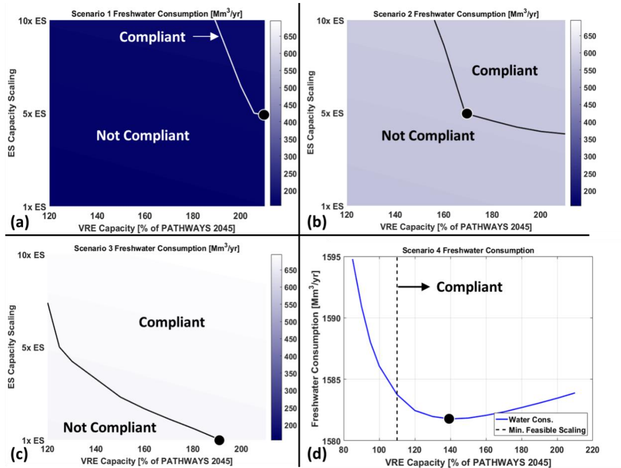
Figure 3 – Freshwater Consumption values for different realizations of each narrative scenario: a) Scenario 1 – Solar/Hydro/Wind Only, b) Scenario 2 – Current Nuclear and Renewable Expansion, c) Scenario 3 – Nuclear and Renewable Expansion, and d) Scenario 4 – Maximize Geothermal and Biogas. The black dot notes the realization with the lowest freshwater consumption value in each scenario. Variable renewable energy capacity is presented as a percentage of levels in the E3 PATHWAYS 2045 study and energy storage capacity is presented as a multiple of levels in the E3 PATHWAYS 2045 study.
