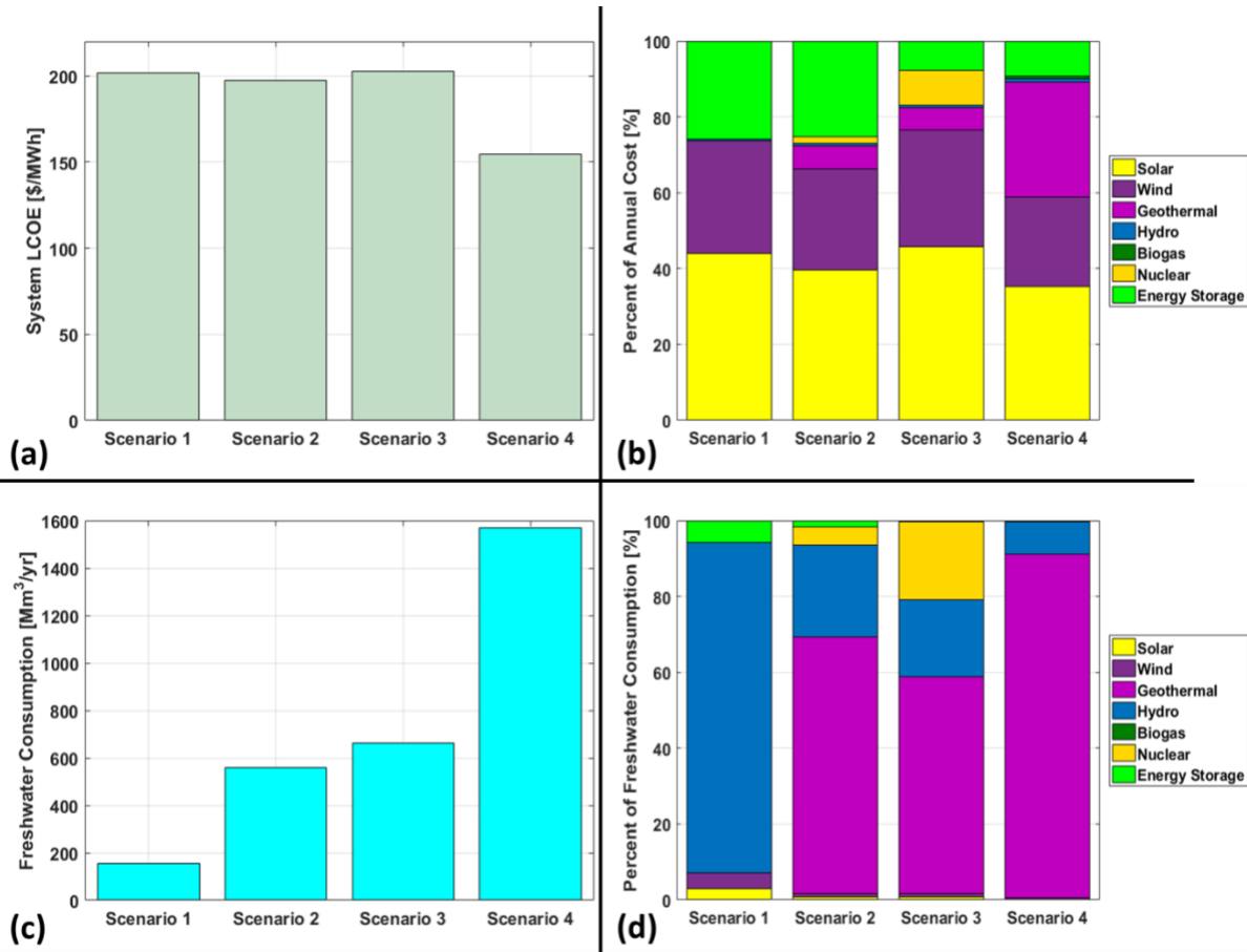
Figure 4 – (a) Systemwide Levelized Cost of Electricity [2017 $/MWh] for the lowest cost realizations in each of the narrative scenarios: Scenario 1 – Solar, Hydropower, and Wind Only, Scenario 2 – Current Nuclear and Renewable Expansion, Scenario 3 – Nuclear and Renewable Expansion, and Scenario 4 – Maximize Geothermal and Biogas. (b) Normalized distribution of annual costs by electric grid resource type for the realizations presented in (a). (c) Annual Freshwater Consumption [Mm 3 /yr] for the lowest freshwater consumption realizations in each of the narrative scenarios. (d) Normalized distribution of annual freshwater consumption by resource type for the realizations presented in (c).
